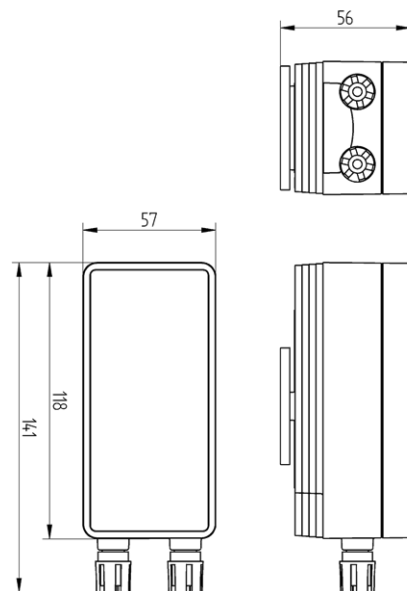
Product dimensions
